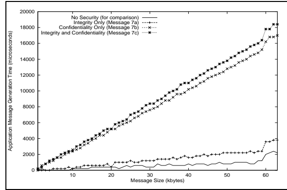
Figure 5: Application Traffic message generation costs - Costs associated with the generation of application messages of varying sizes and security guarantees.
