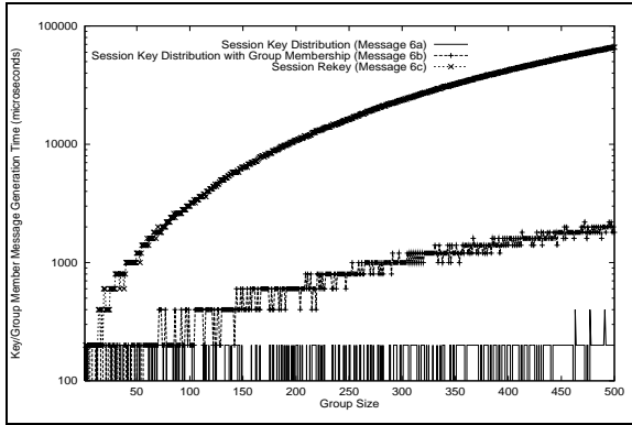
Figure 4: Group Membership/Session Key message generation costs - Costs associated with the message generation of groups of varying sizes and semantics.
