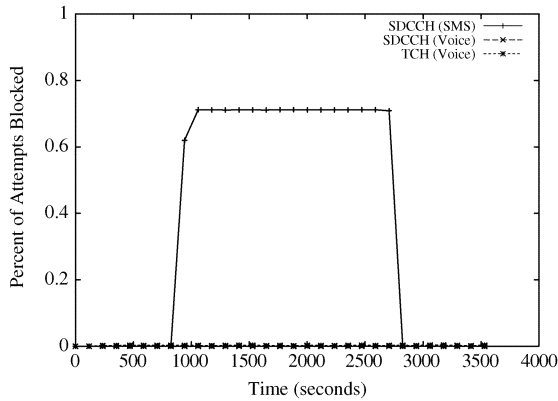
Fig. 19. Blocking for a sector implementing DCA.
