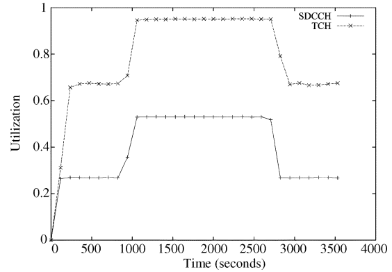
Fig. 6. Channel utilization characteristics of a network under emergency conditions (100 K calls/hr, 276 K msgs/hour).
