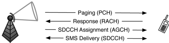
Fig. 2. Overview of SMS message delivery on the wireless or air interface. Incoming voice calls would follow a similar procedure except that they would receive a TCH after using the SDCCH.
