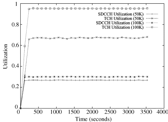
Fig. 4. Channel utilization in a network with a variety of traffic intensities.
