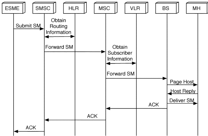
Fig. 1. High level description of SMS delivery in an SS7 network.
