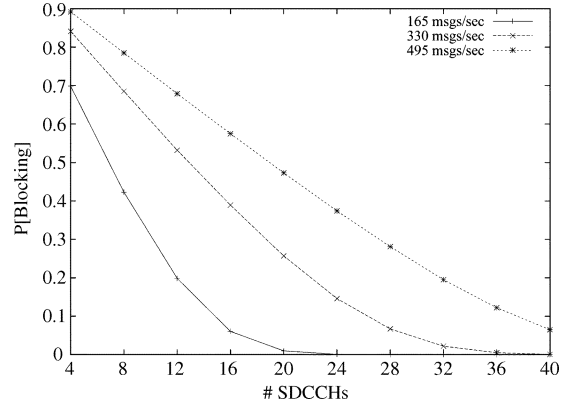
Fig. 10. Probability of an incoming call/message blocking in a sector for a varying number of SDCCHs.
