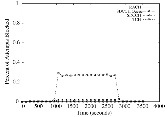
Fig. 5. Blocking characteristics of a network under emergency conditions (100 K calls/hr, 276 K msgs/hour).
