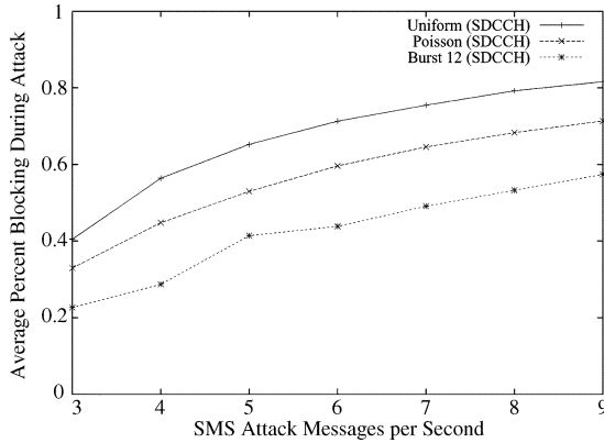
Fig. 7. Blocking probability for traffic exhibiting uniform, Poisson and bursty arrival patterns over varying attack strengths.
