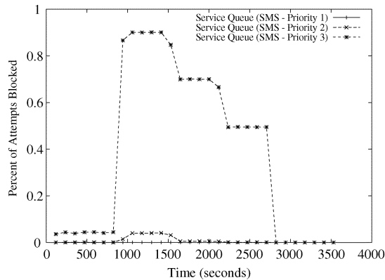
Fig. 21. Blocking for a sector implementing both WRED and DRP.
