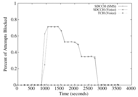
Fig. 17. Blocking for a sector implementing DRP.
