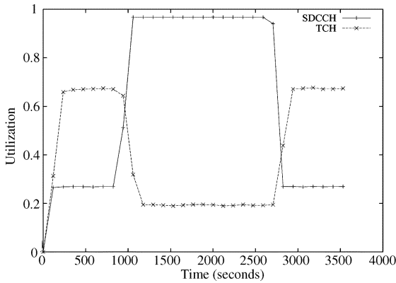
Fig. 8. Utilization of SDCCHs and TCHs for an attack exhibiting a Poisson interarrival at a rate of 495 messages/second.
