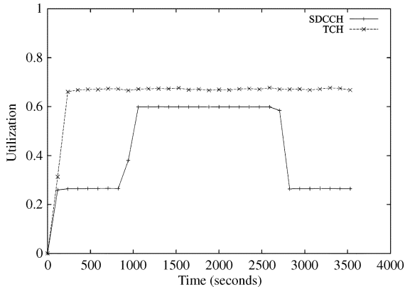
Fig. 16. Channel utilization under SRP.
