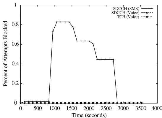
Fig. 22. Blocking for a sector combining DRP and SRP.
