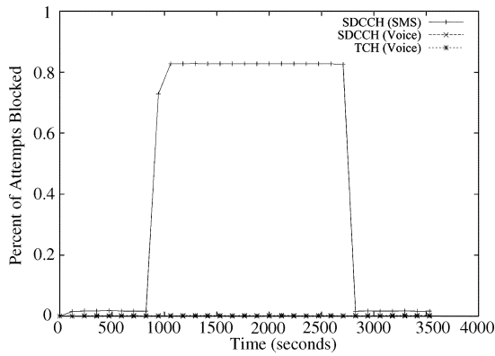
Fig. 15. Blocking for a sector implementing SRP.
